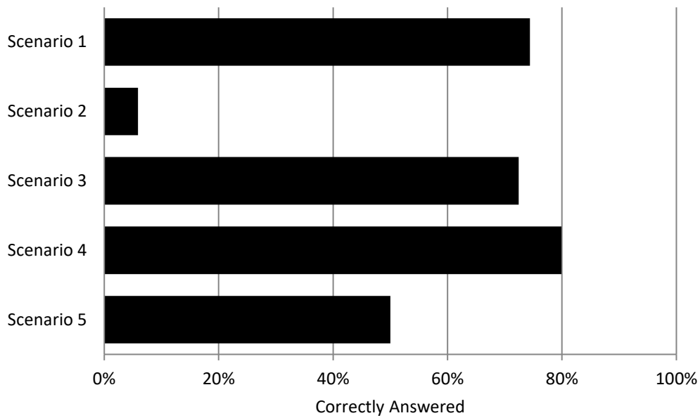
Figure 2. Percentage of Correct Answers
